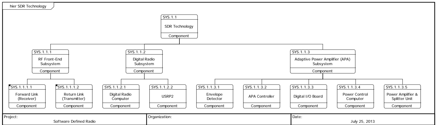
Figure 6. High level SDR Technology Component Hierarch
