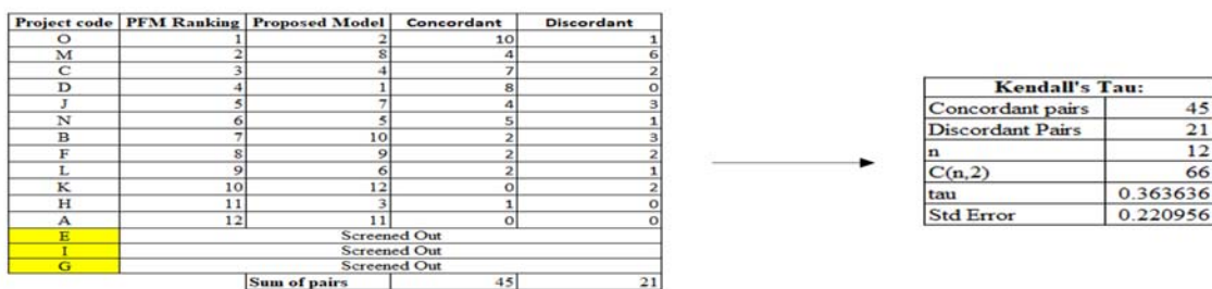
Figure 4: Kendall’s Tau Result relative to Proposed Model and PFM Ranking
