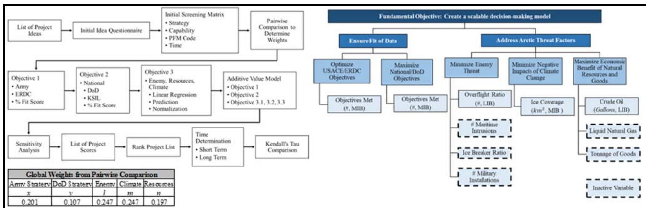
Figure 3. Proposed Methodology Process, Value Model, and Global Weights
